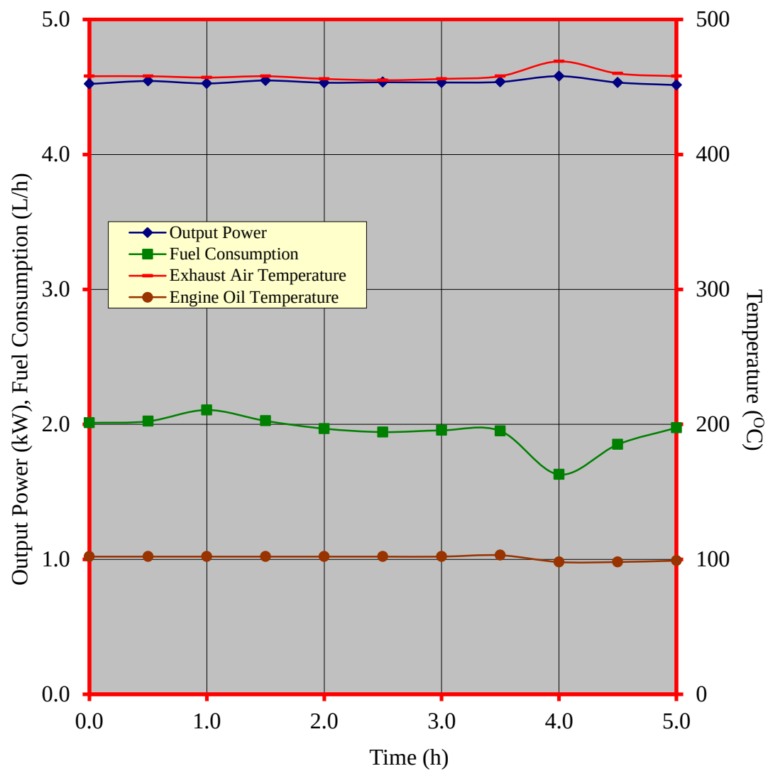
Figure 4. Performance characteristic curves during the continuous running test of the CHANG HONG R180 diesel engine
