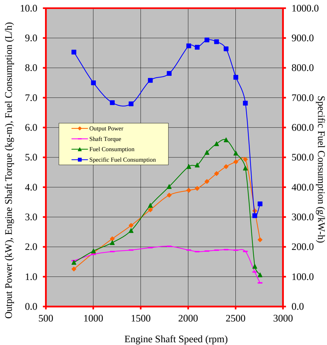
Figure 3. Performance characteristic curves of the CHANG HONG R180 diesel engine
