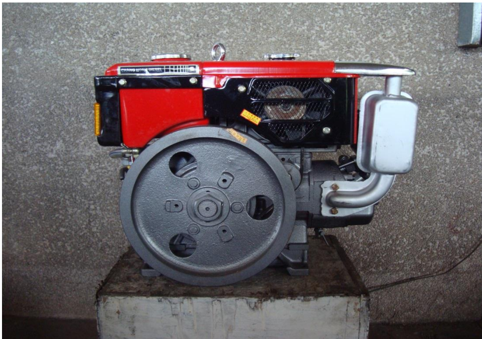
Figure 1. CHANG HONG R180 Diesel Engine
